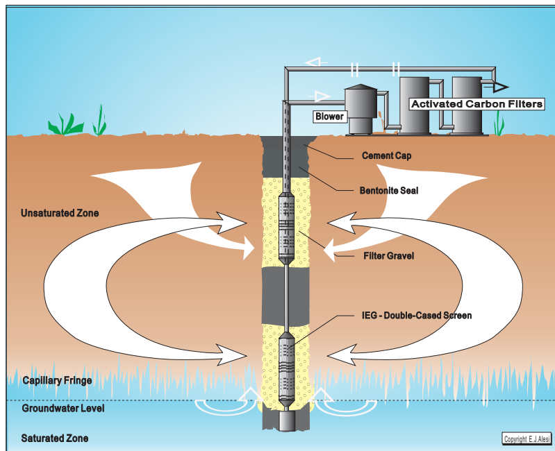
IEG Soil Air Circulation-Vacuum Vapour Extraction System (IEG SAC-VVE Process)
